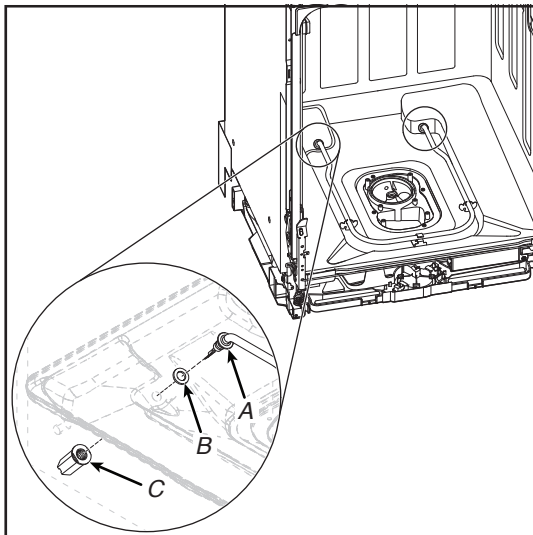
A. Heater Element Assembly B. Heater Washer C. Heater Element Nut
